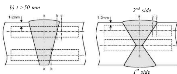
Fig. 6.4.4.4-2 Location of V-notch for butt weld of normal heat input (heat input \leq 50 kJ/cm):
