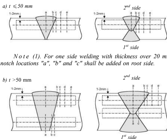
Fig. 6.4.4.4-3 Location of V-notch for butt weld of high heat input (heat input > 50 \text{ kJ/cm} ):
